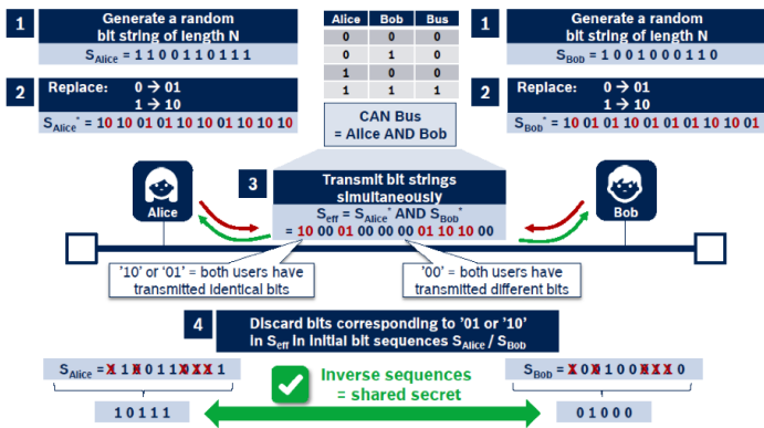
Figure 2: Basic idea for easy key agreement in CAN networks by means of the novel "Plug-and-Secure Communication for CAN" approach (Photo: Bosch)
