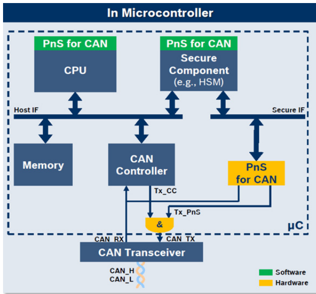
Figure 3: Two possible implementation options (Photo: Bosch)
