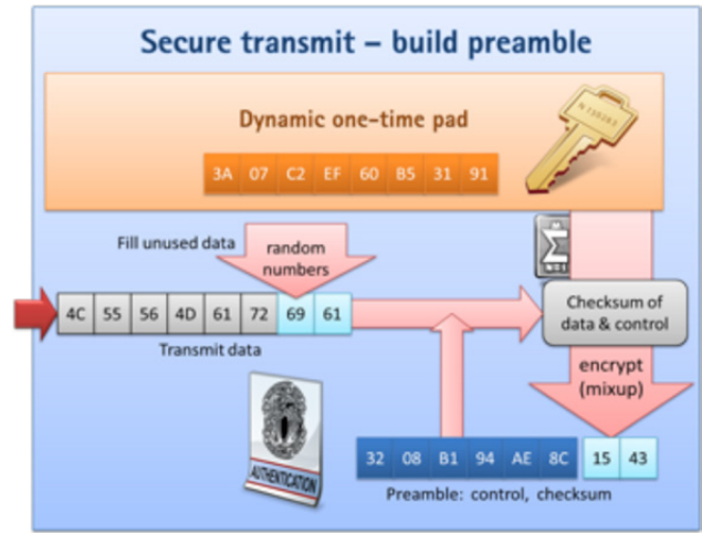
Figure 9: Secure transmit with preamble (Photo: Esacademy)
